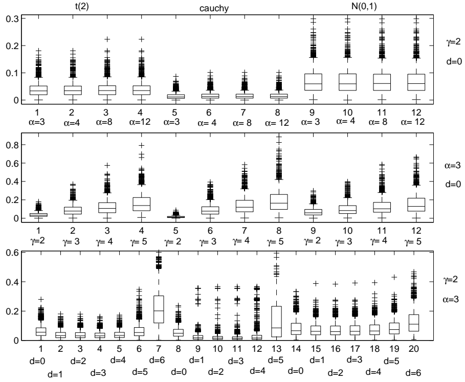
Figure 5: Boxplots of AAE of WLADe with different \alpha , \gamma and d for model (4.1) .
