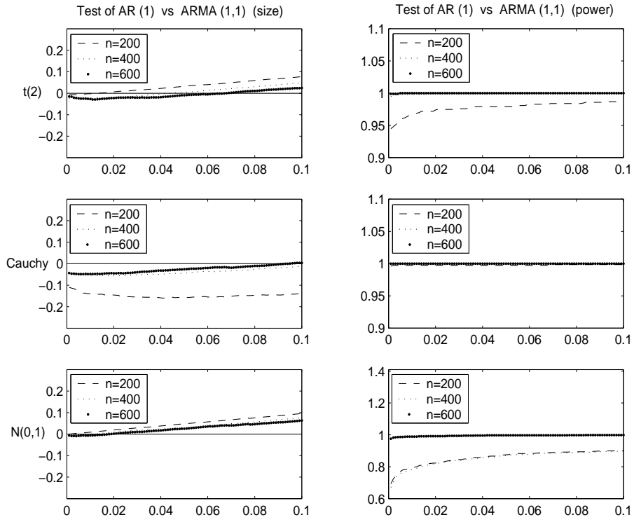
Figure 6: Simulation results for the Wald test. Differences between approximated P -value and the nominal significance level is plotted against the nominal level. The data were generated from (4.1) with (\phi_1, \theta_1) = (0.3, 0) for the three panels on the left, and (\phi_1, \theta_1) = (0.3, 0.5) for the three panels on the right.
