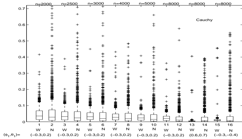
Figure 4: Boxplots of the AAE of WLADE and Gauss-Newton estimator for model (4.1) for large sample case.
