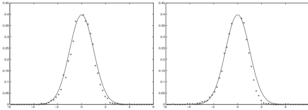
Figure 1: Estimated values ( \times ) for the density functions of the normalized \hat{\phi}_1 (left panel) and \hat{\theta}_1 (right panel), together with their asymptotic limit — the N(0,1) density (solid curves) for model (4.1) with t_2 innovations.
