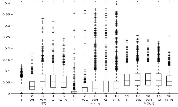
Figure 3: Boxplots of the AAE of LADE, WLADE, Whittle estimator, QMLE and Gauss-Newton estimator for model (4.1).
