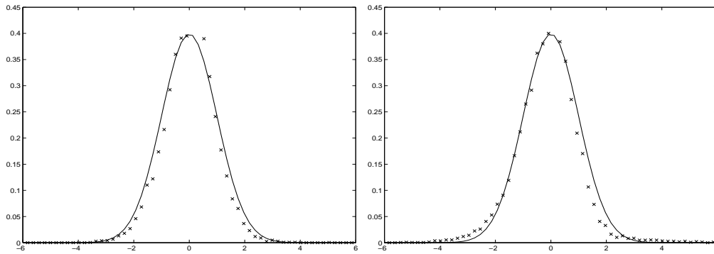
Figure 2: Estimated values ( \times ) for the density functions of the normalized \hat{\phi}_1 (left panel) and \hat{\theta}_1 (right panel), together with their asymptotic limit — the N(0,1) density (solid curves) for model (4.1) with Cauchy innovations.
